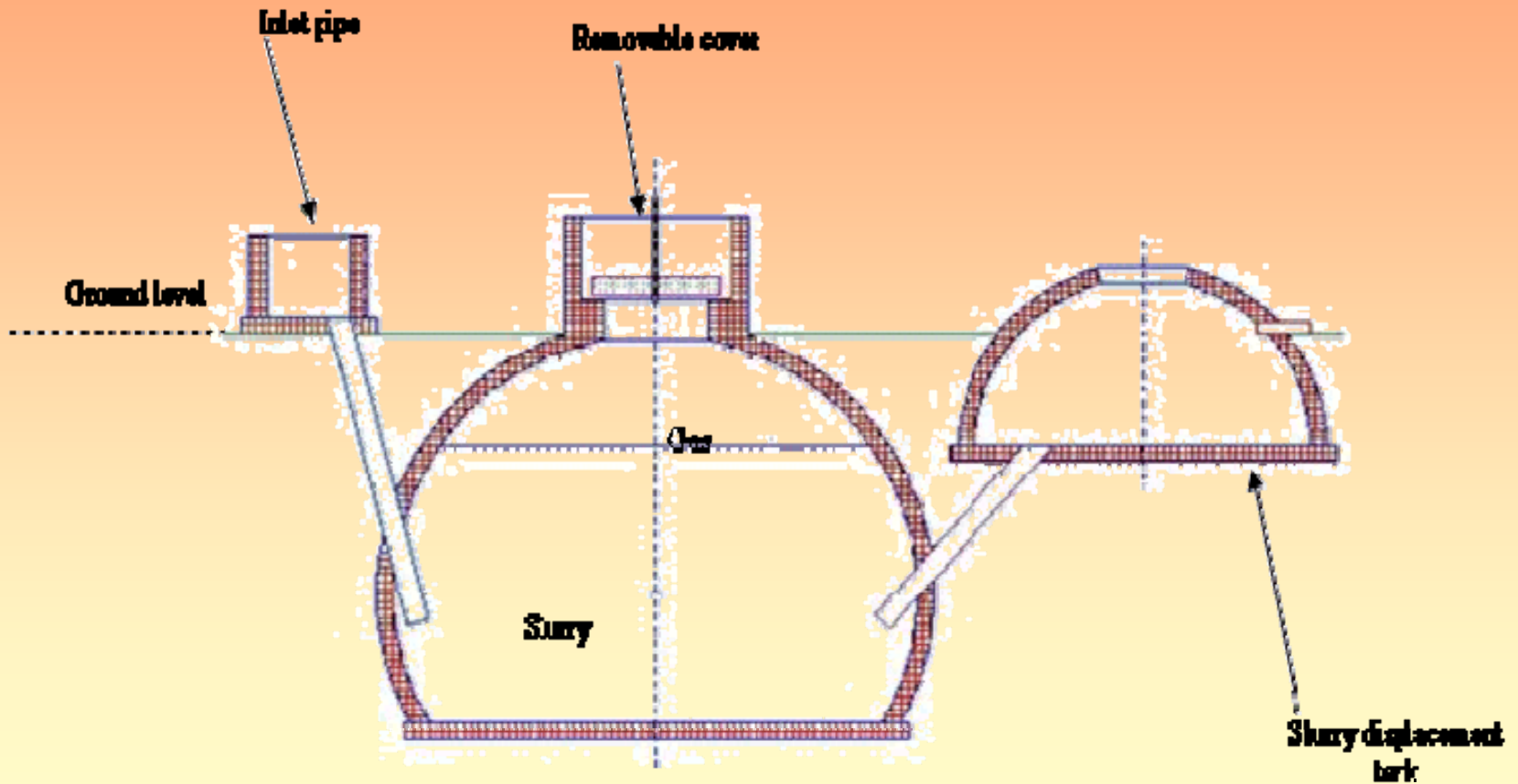
Figure 3: Spherical shaped fixed - dome plant
